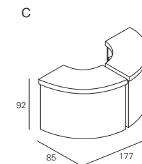
05540 Helix Curve 05540 Helix Curve
